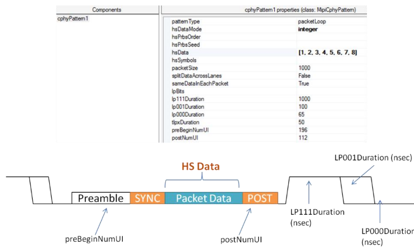
Figure 6: Global timing parameter control from within the cphyPattern component.
