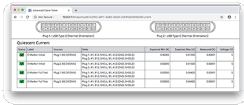
Figure 34 : Web Application - Individual Test Report - Quiescent Current Section
