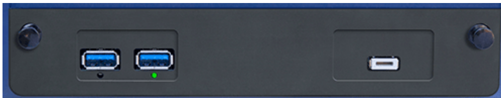
Figure 12 : Multiple Connector Module
