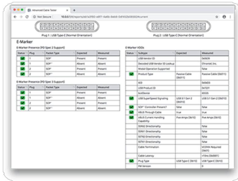
Figure 32 : Web Application - Individual Test Report - E-Marker Section
