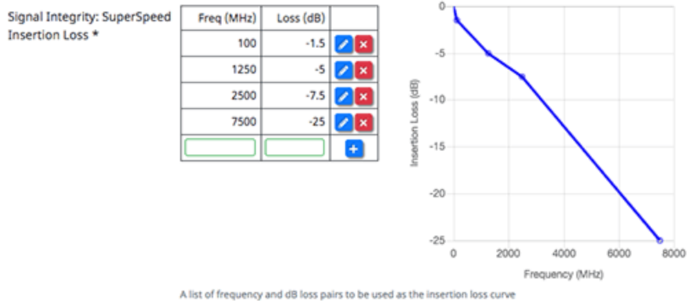
Figure 39 : Web Application - Individual Profile - Insertion Loss Field
