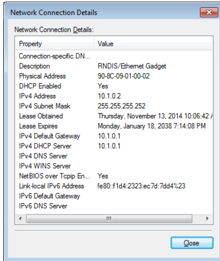
Figure 8 : Windows Connection Details.
