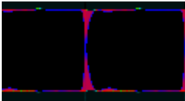
Figure 2: USB 2.0 Eye Diagram at 480 Mbps
