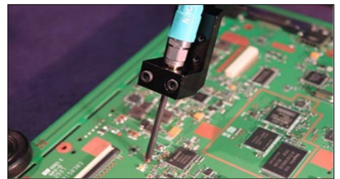
Single-Ended Fixed Pitch Probe System. The probe is attached to an adapter and to the end of a Probe Positioner arm. Several fixed pitches and bandwidths are available.
